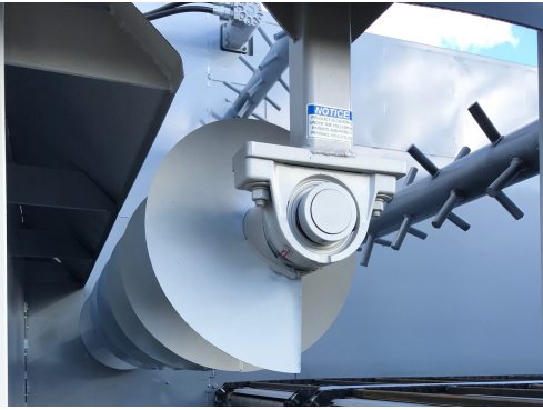
EQUALIZER AUGER
